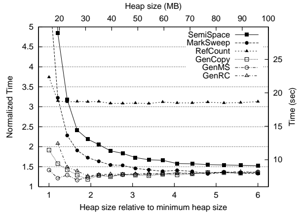
Figure 4. JMTk Collectors on _202_jess
