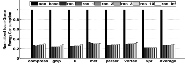
Figure 7: Normalized issue queue energy
